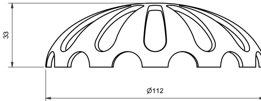
DOMED URINAL TOP 100mm
