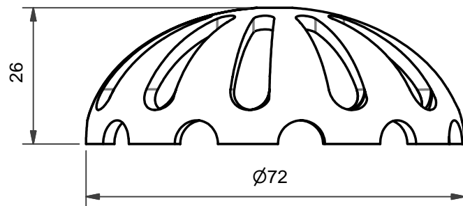
DOMED URINAL TOP 50mm & 65mm
